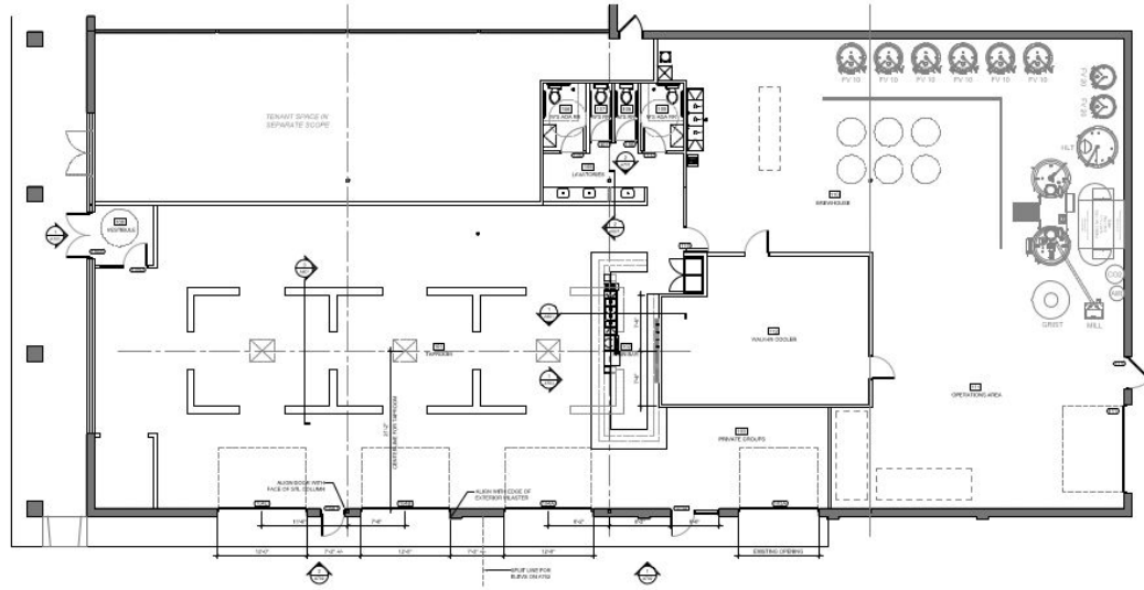
1 FLOOR PLAN A101 3/16" = 1'-0"
